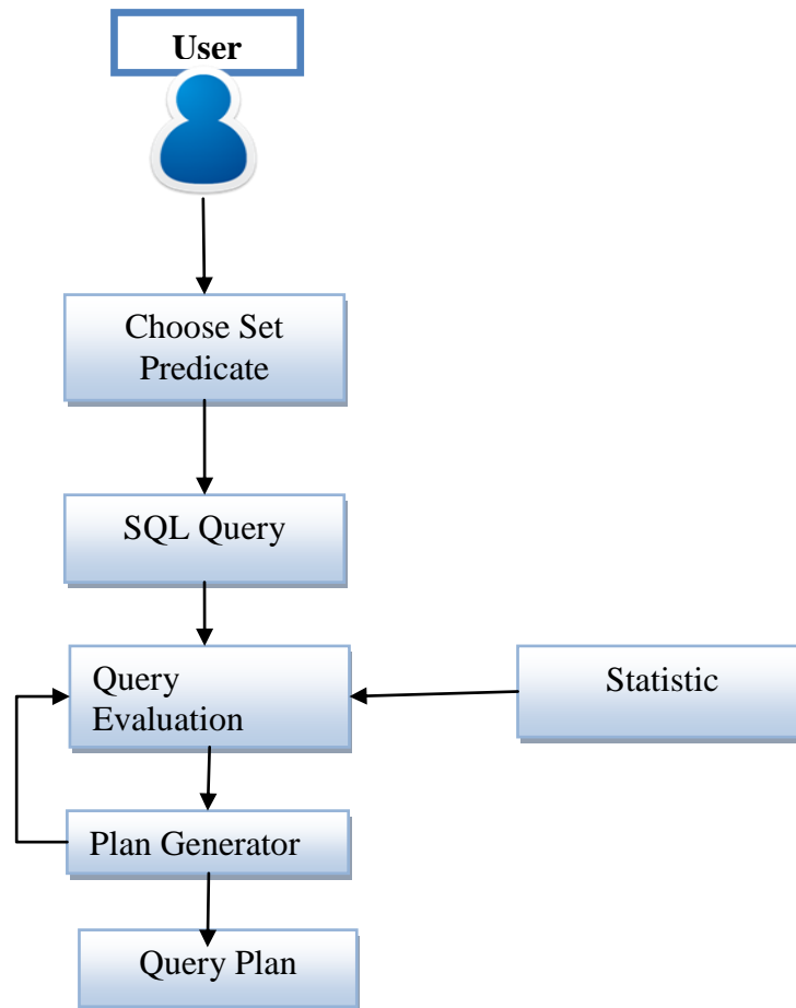
Figure 1 Overall Architecture
