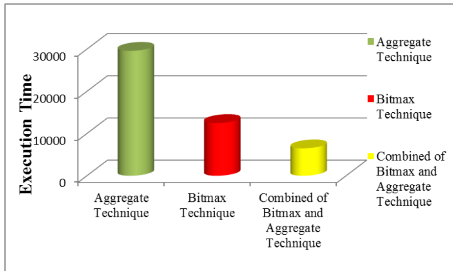
Figure6. Result Analysis
